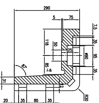
SEC B-B SCALE 1:5
