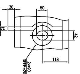
VIEW M SCALE 1:5
