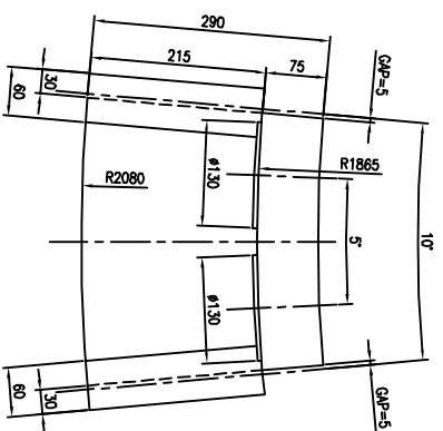
BACK VIEW SCALE 1:5
