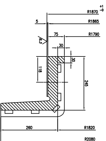
SEC A-A SCALE 1:5
