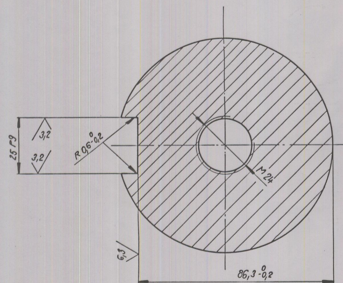
A - A (1:1)
