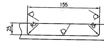
VIEW M
