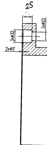
VIEW M
