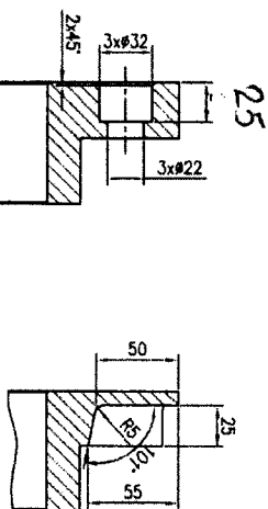
VIEW M
