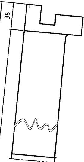
View C
